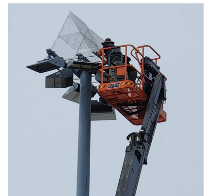
Double Crossarm
